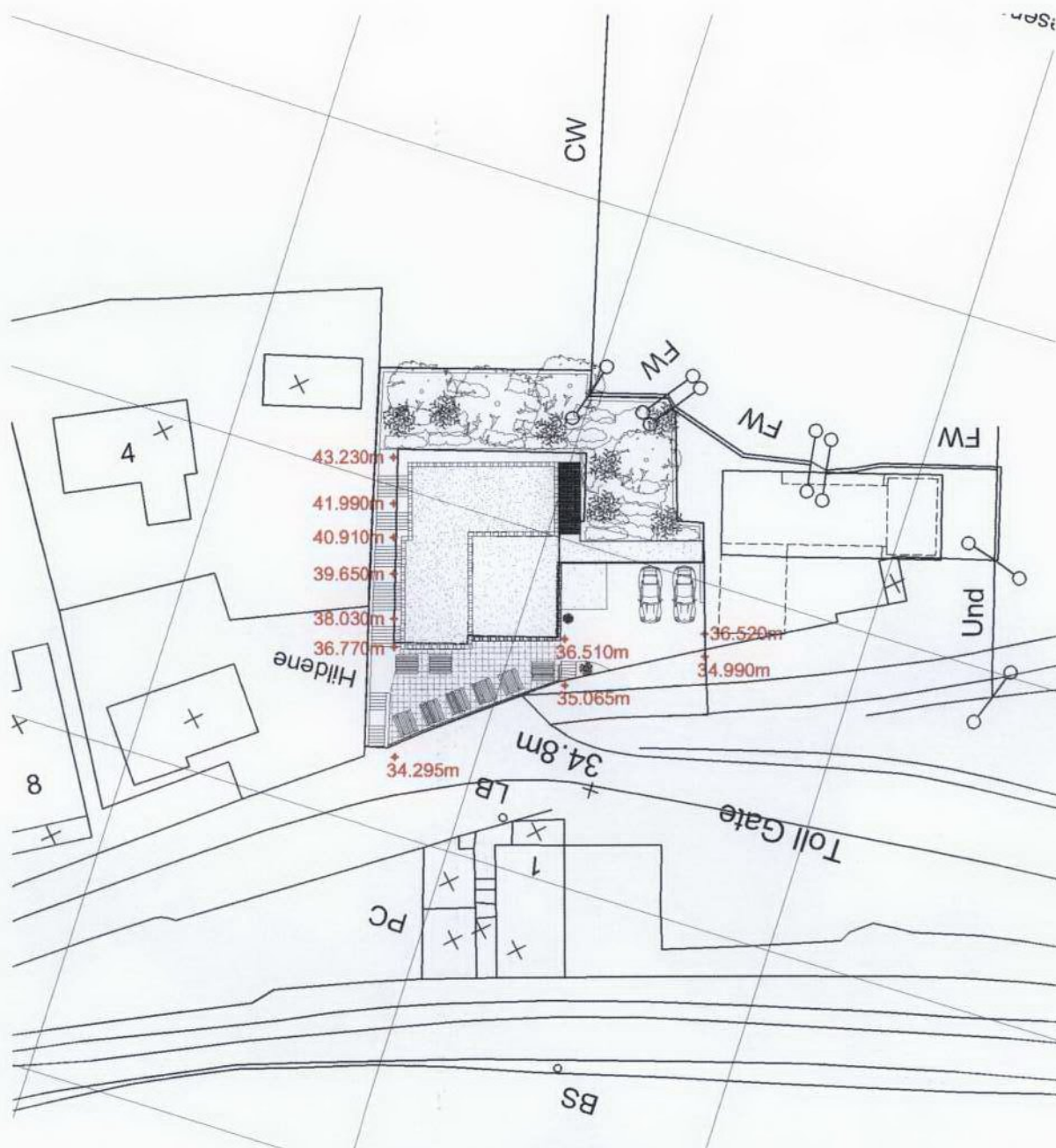
EXISTING SITE SURVEY 1:500
